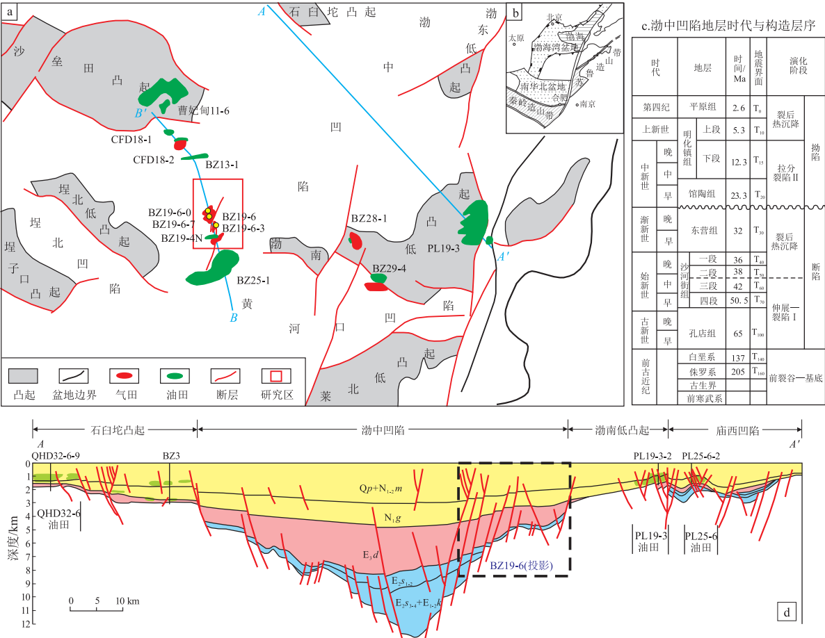
图 1 渤海湾盆地渤中凹陷平面及剖面结构 Fig.1 Plane and section structure of Bozhong Sag, Bohai Bay Basin
