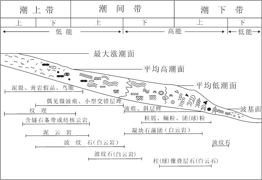
图 2 雾迷山组沉积相模式图(据周书欣,1979,有改动) Fig.2 Sedimentary facies model of Wumishan Formation(modified after Zhou Shuxin,1979)
