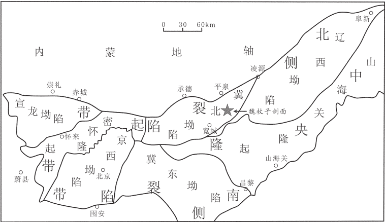
图 1 燕山地区中元古界实测剖面位置示意图(据王铁冠,1980,有改动) Fig.1 Location of Mesoproterozoic measured section in Yanshan area(modified after Wang Tieguan,1980)
