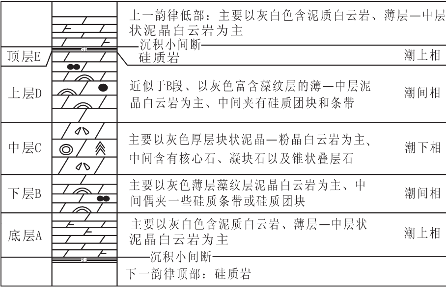
图 3 雾迷山组沉积韵律模式图(据黄学光,2006,有改动) Fig.3 Deposition rhythm pattern of Wumishan Formation(modified after Huang Xueguang,2006)
