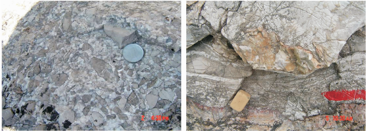
图 5 第一段 8 层的岩溶角砾岩(左)和 48 层顶部冲刷面(右) Fig. 5 8-layer karst breccia (left) and erosion surface at the top of 48-layer (right)
