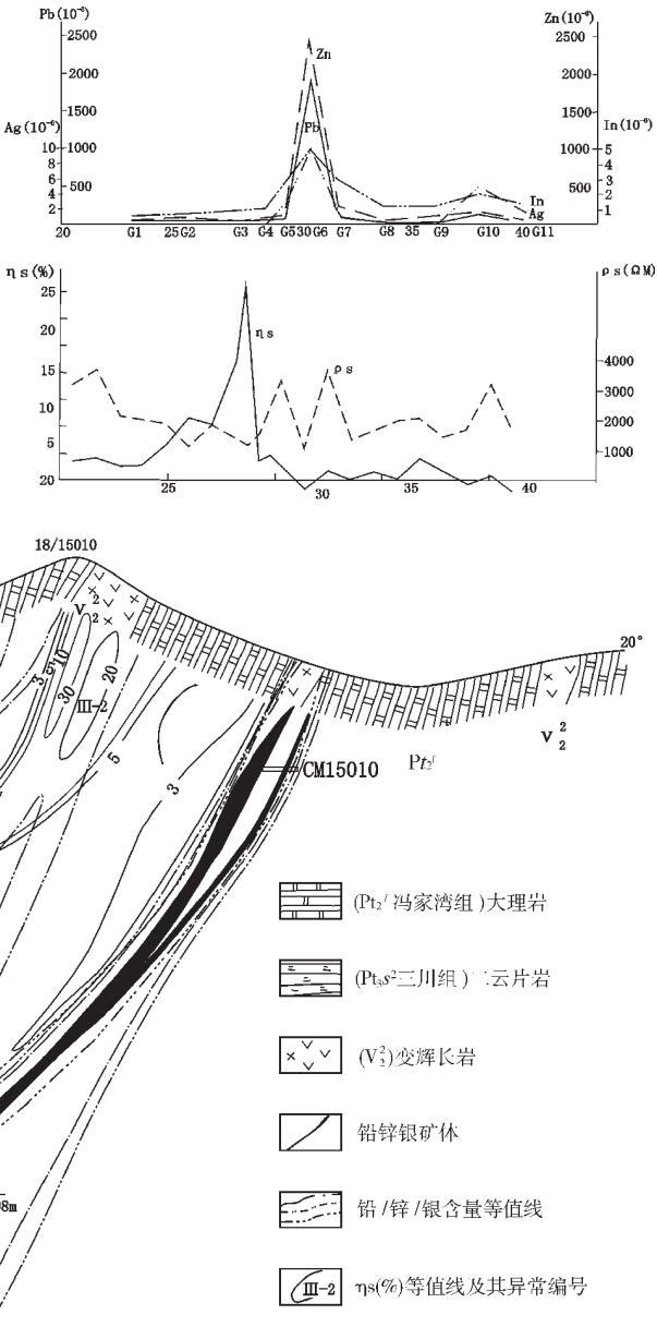
图 5 百炉沟矿区 S150 矿脉综合剖面图 Fig. 5 Integrated section of ore vein S150 of the Bailugou mining area
