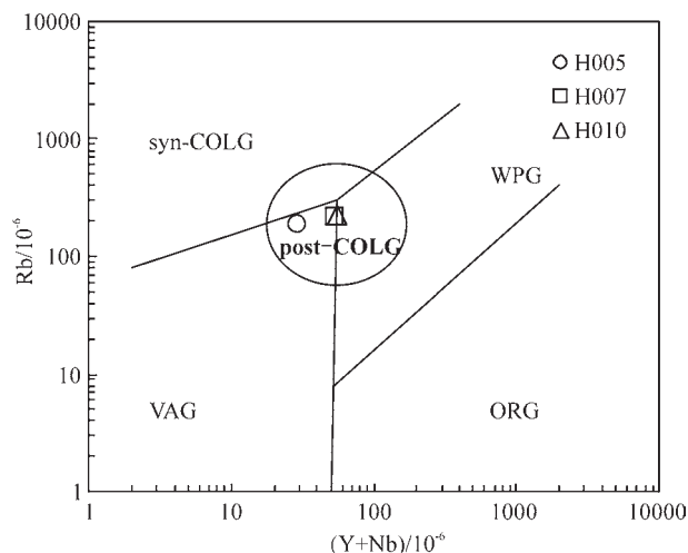
图9 (Y+Nb)-Rb 图解(底图据文献[18]) ORG—洋脊花岗岩; WPG—板内花岗岩; VAG—火山弧花岗岩; syn-COLG—同碰撞花岗岩; Post-COLG—后碰撞花岗岩 Fig.9 (Y+Nb)-Rb diagram of volcanic rocks in the study area (after Reference [18]) ORG—Ocean ridge granite; WPG—Intraplate granite; VAG—Volcanic arc granite; Syn-COLG—Syn-collision granite; Post-COLG—collision granite
