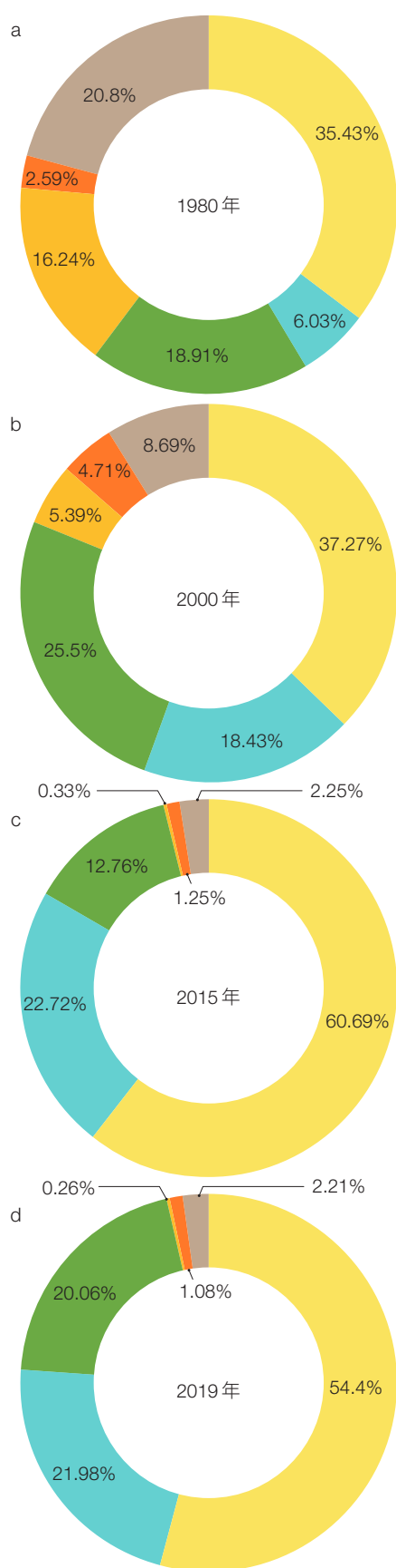
图2 1980—2019年我国东北地区粮食种植结构变化 Figure 2 Changes of grain planting structure in Northeast China from 1980 to 2019
