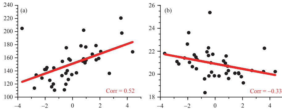
Figure 7. (a) The scatter diagram of summer NCCVI (x-axis) and regional average monthly total precipitation (y-axis) in Northeastern China. (b) is similar to (a), but for the scatter diagram of summer NCCVI (x-axis) and regional average monthly surface temperature at 2 m (y-axis). The red lines indicate linear regressions of NCCVI on precipitation and surface temperature, respectively. The correlation coefficients between NCCVI and the regional average of precipitation or surface temperature are 0.52 and -0.33 , respectively; the results are both statistically significant at the confidence level of 95%.
