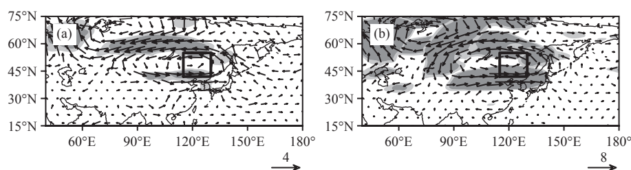
Figure 4. The composite differences of horizontal winds (vectors, units: \text{m s}^{-1} ) at (a) 850 hPa and (b) 300 hPa between strong NCCVI years and weak NCCVI years. The light (dark) gray shaded area indicates results statistically significant at the confidence level of 90% (95%). The black boxes indicate Northeastern China.
