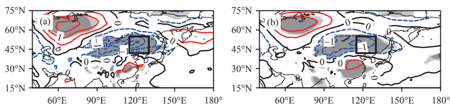
Figure 5. The composite differences of temperature (contours, units: ^{\circ}\text{C} ) at (a) 850 hPa and (b) 700 hPa between strong and weak NCCVI years. The light (dark) gray shaded area indicates results statistically significant at the confidence level of 90% (95%). The black boxes indicate Northeastern China.
