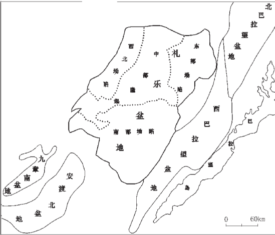
图 1 礼乐盆地位置及构造区划图 Fig. 1 Map showing the location and tectonic divisions of the Lile basin
