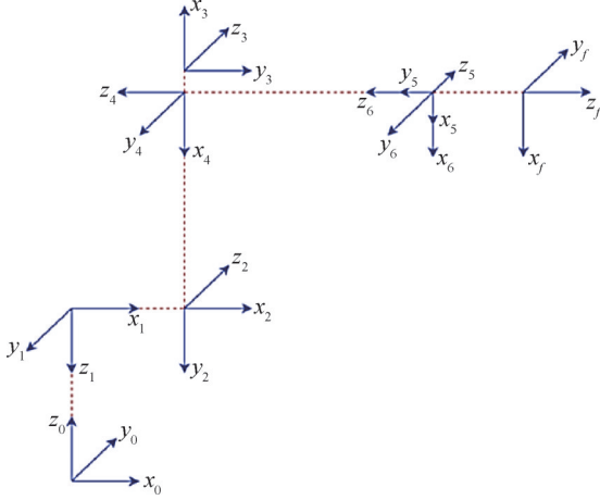
Fig.2 KR10R1420 Robot with Coordinate System
