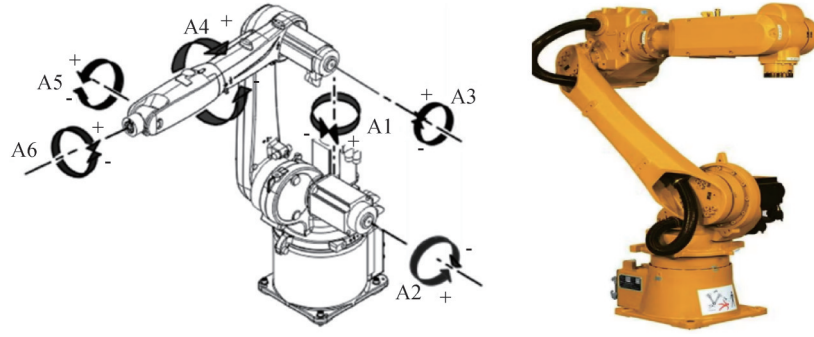
Fig.1 KR10R1420 Robot with six-degree-of-freedom
