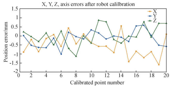
Fig.5 X, Y and Z axis errors after calibrating the robot
