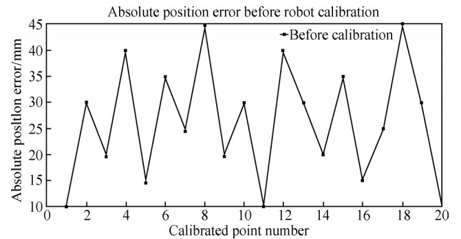
Fig.6 Absolute position error before robot calibration
