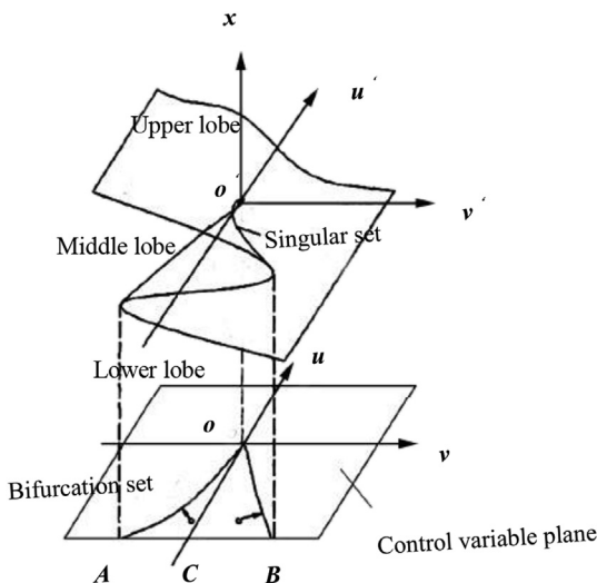
Fig. 1. Equilibrium surface and bifurcation set of cusp catastrophe model [16].
