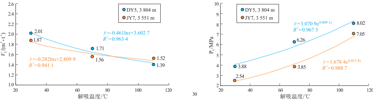
图 6 川东南地区 JY7、DY5 井龙马溪组深层页岩样品 Langmuir 体积、Langmuir 压力与解吸温度的关系 Fig.6 Relationship between V_L , P_L and temperatures of deep shale samples from Longmaxi Formation in wells JY7 and DY5 in southeastern Sichuan Basin
