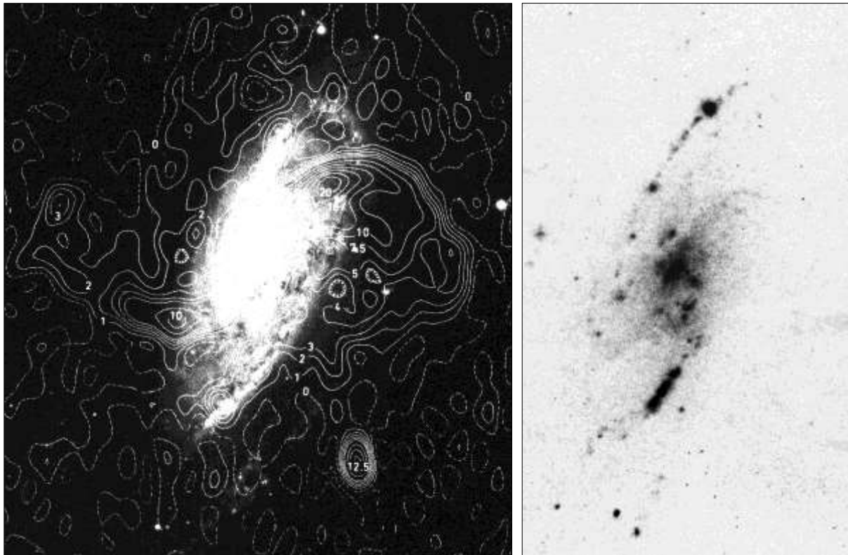
Figure 7: NGC 4258. On the left an optical image with the radio continuum contours superimposed and on the right a photograph taken in the light of ionized hydrogen ( H\alpha ), taken by French observers and published some years before (after van der Kruit, Mathewson and Oort, 1972 ).
