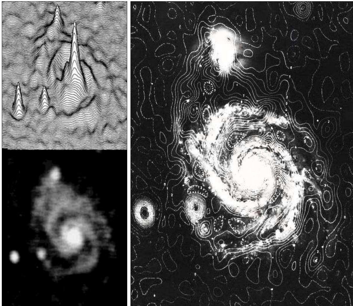
Figure 6: Westerbork observations of the continuum radiation of the Whirlpool Galaxy M51. On the top-left a so-called ruled surface plot and below that an intensity representation produced by Walter Jaffe on a cathode-ray tube. On the right brightness contours superposed on an optical image (after Mathewson, van der Kruit and Brouw, 1972 ).
