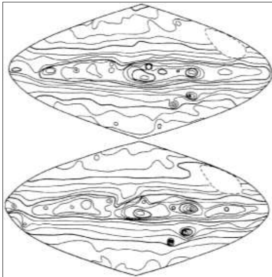
Figure 17: Full-sky surface brightness distribution of the Galaxy after removal of stars with m < 6.5 , from Pioneer 10 in the red (top) and blue. The angular resolution is 8°. The direction towards the Galactic Center is in the middle of the pictures and the north pole at the top. Galactic longitude increases towards the left. The contour unit is 0.25 mag arcsec -2 ; the faintest thick one in the upper part corresponds to about 24 V-mag arcsec -2 and in the lower part to about 24 B-mag arcsec -2 . The missing part is the direction towards the Sun as seen from Jupiter around Pioneer 10 encounter. Note the Magellanic Clouds on the lower right (after van der Kruit, 1984 ).
