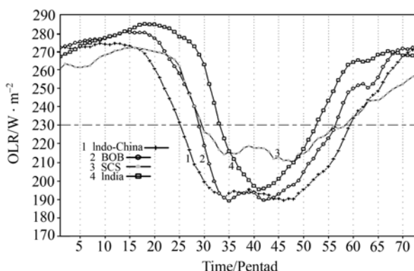
Fig. 4. The time series of area-averaged OLR associated with the key regions of the ASM. Abscissa indicates pentads. The horizontal dash line represents the value of OLR equal to 230 W m^{-2} . 1, southern Indochina Peninsula; 2, the eastern Bay of Bengal (BOB); 3, the SCS; 4, indicates the Indian subcontinent.
