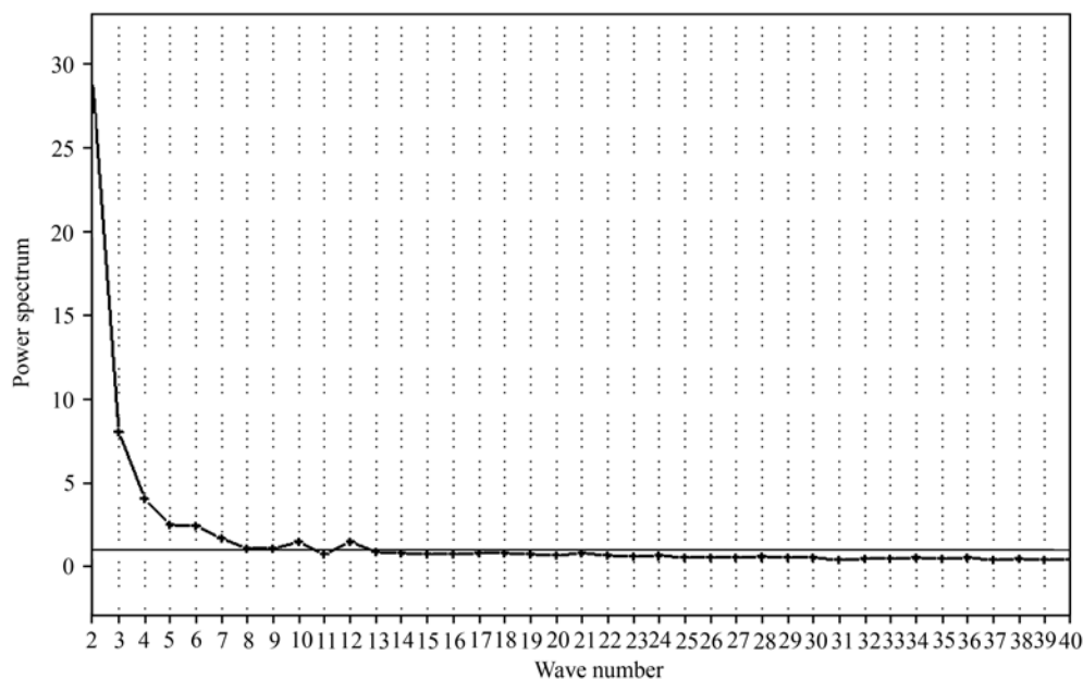
Fig. 1. The significant test associated with the mean of the dispersible power spectrum of climatological OLR averaged over Asian monsoon region ( 10^{\circ}\text{S} – 40^{\circ}\text{N} , 40^{\circ} – 150^{\circ}\text{E} ). Abscissa indicates wave numbers (waves 2 to 40). Vertical coordinate denotes F value of the dispersible power spectrum. Horizontal solid line represents F=1.0 .
