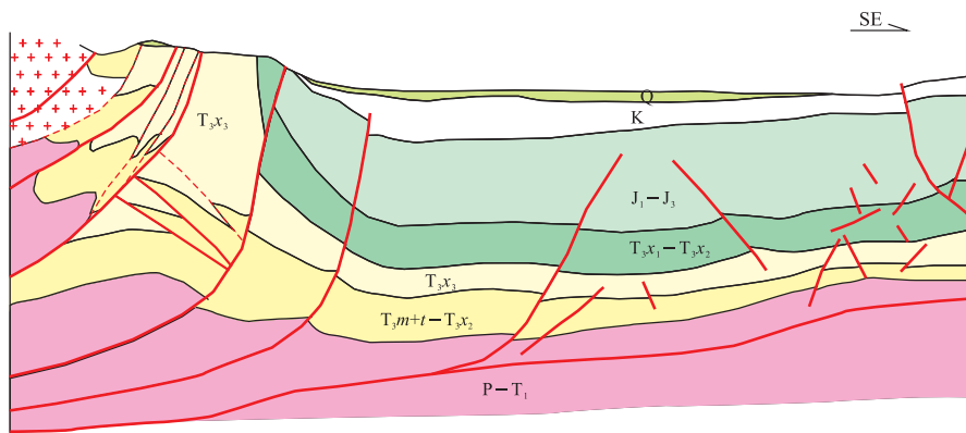
图 4 川西龙门山前构造剖面 Fig.4 Structural section of Longmen Mountain front, western Sichuan Basin
