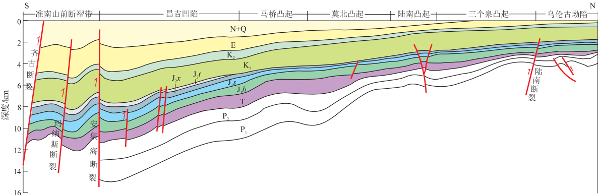
图2 准噶尔盆地中部构造剖面 Fig.2 Structural section of central Junggar Basin
