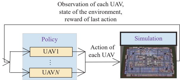
图 3 仿真平台数据交互过程 Fig.3 Data interaction process of simulation platform
