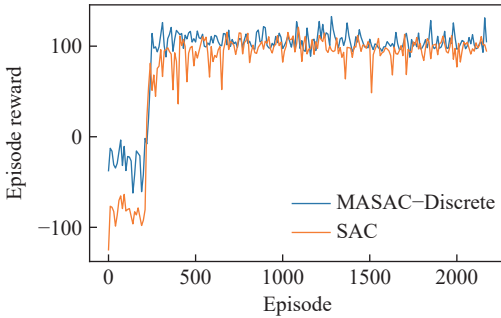
图 6 回合奖励曲线 Fig.6 Episode reward curve
