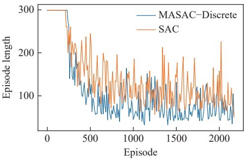
图 5 回合长度曲线 Fig.5 Episode length curve
