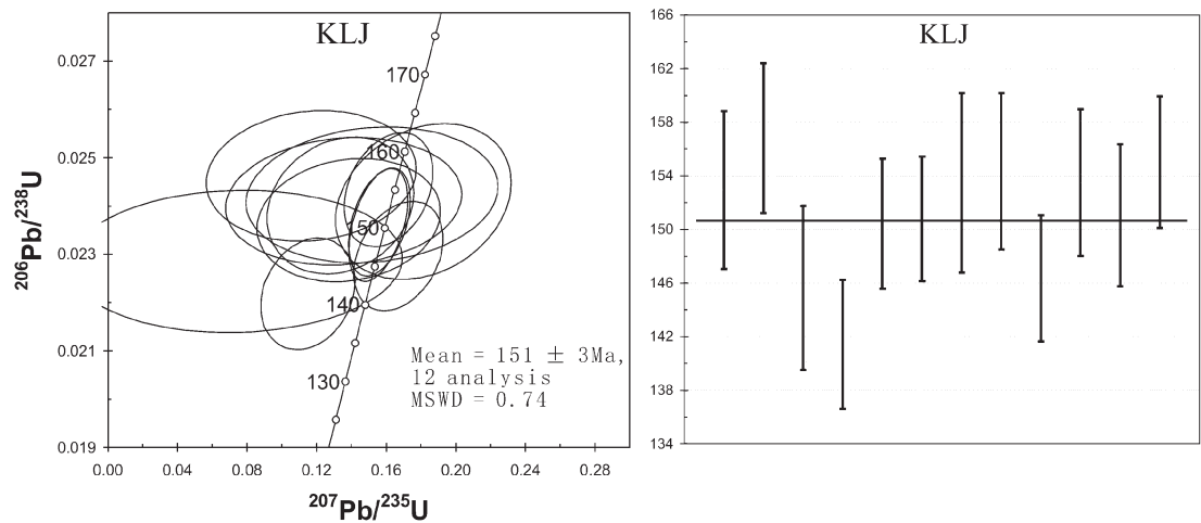
图 3 开岭脚花岗闪长岩中锆石 U-Pb 谐和图(12 个测点) Fig.3 U-Pb concordia diagram of zircons from Kailingjiao granodiorites (12 analytical spots)
