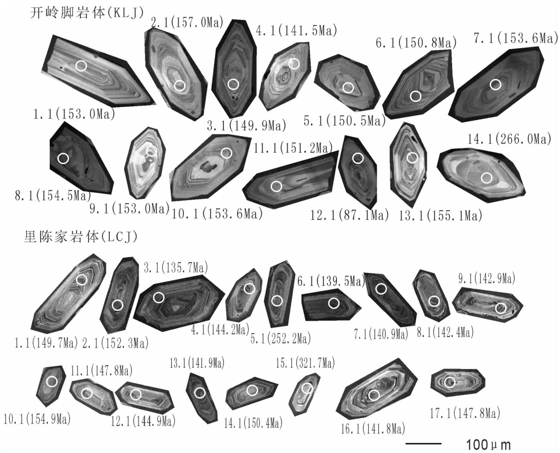
图 2 开岭脚、里陈家花岗闪长岩体中代表性锆石的阴极发光图像 Fig.2 Cathodoluminescence images of representative zircons from Kailingjiao and Lichenjia granodiorites
