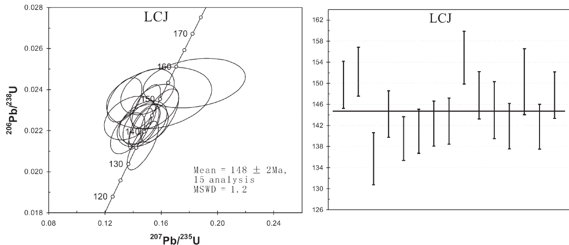
图 4 里陈家花岗闪长岩中锆石 U-Pb 谐和图(15 个测点) Fig.4 U-Pb concordia diagram of zircons from Lichenjia granodiorites (15 analytical spots)
