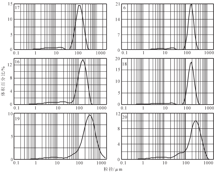
图 1 松花江哈尔滨段河流冲积物粒度分布曲线图 (图中左上角数字表示样品号) Fig.1 Curves of grain-size distribution of river alluvium in the Harbin reach of the Songhuajiang River (The number at the upper-left corner in the figure denotes sample No)
