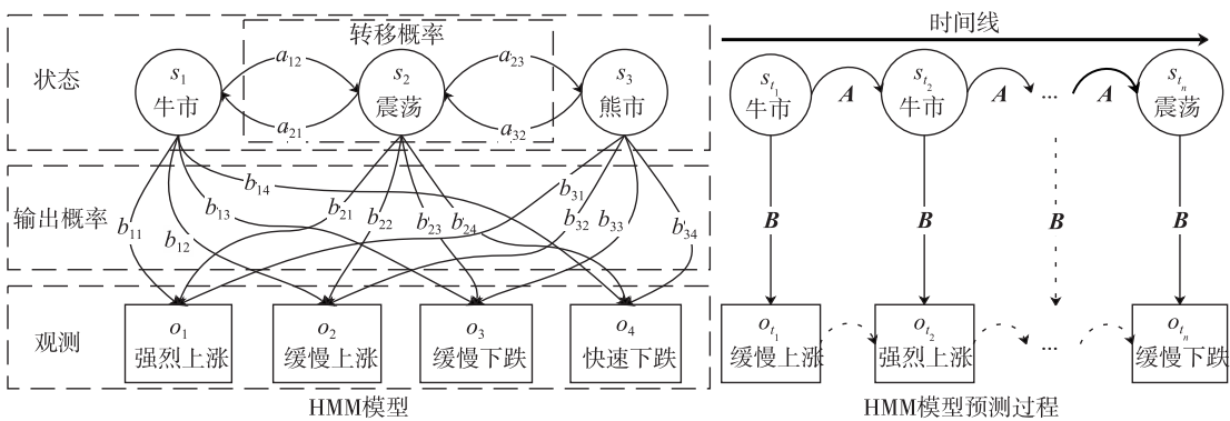
图 1 HMM 量化金融示例 Fig. 1 Example of HMM on quantitative finance
