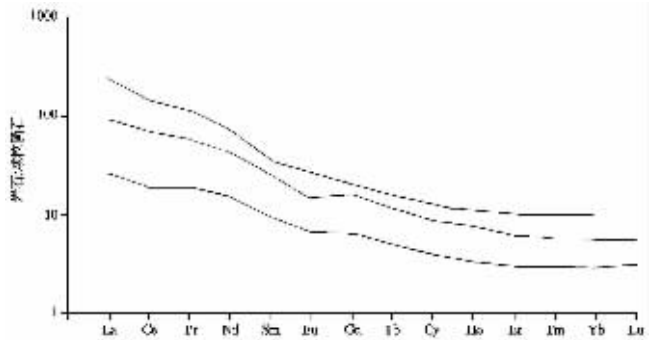
图6 普朗矿区酸性斑岩类稀土配分曲线(Boynton, 1984) Fig.6 REE distribution patterns for acid porphyry in the Pulang ore district (after Boynton, 1984)
