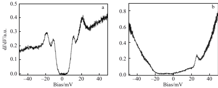
图4 MBE制备1-UC和2-UC FeSe薄膜的STS图 Fig.4 STS images of 1-UC (a) and 2-UC (b) FeSe films fabricated by MBE [10]
