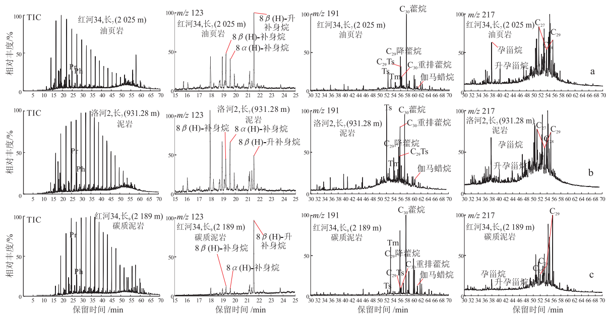
图3 鄂尔多斯盆地南部延长组不同岩性烃源岩饱和烃生物标志物质量色谱 Fig.3 Mass chromatograms of saturated hydrocarbon biomarkers of different lithologic source rocks from Yanchang Formation in southern Ordos Basin
