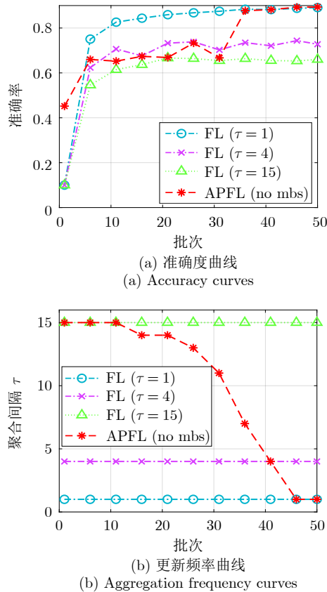
图 10 F-MNIST 自适应模型更新间隔消融实验曲线 Fig.10 Experiment curves of the adaptive model aggregation interval on F-MNIST
