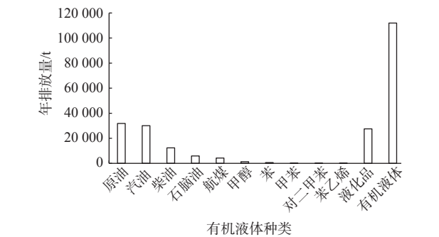
图 1 10 种挥发性有机液体装载源项 VOCs 的排放量 Fig. 1 VOCs emissions of volatile organic liquids loading and ten typical volatile organic liquids loading
