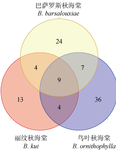
图 1 3 种秋海棠挥发性成分韦恩图分析 Fig. 1 Venn diagram analysis of volatile components in three Begonia species
