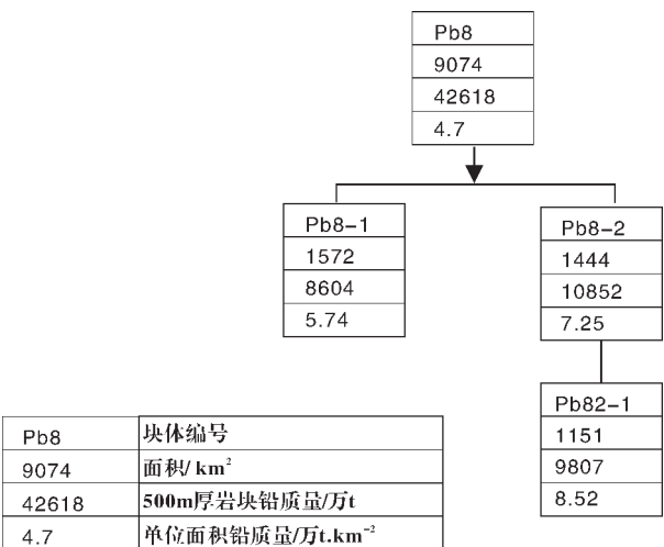
图 2 成县—太阳寺铅地球化学块体内部结构谱系图 Fig. 2 Hierarchal dendrogram of the internal structure of the Chengxian-Taiyansi lead geochemical block
