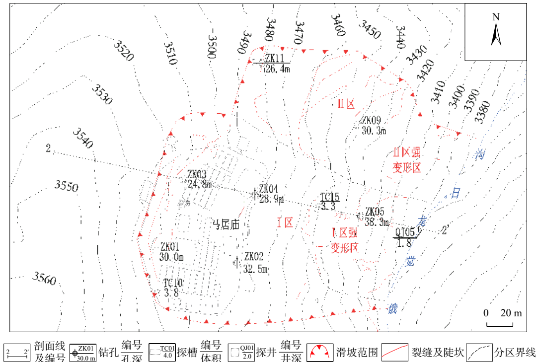
图 2 马居滑坡工程地质平面图 Fig. 2 Engineering geological plane map of Maju landslide
