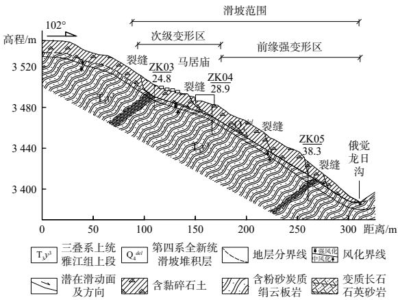
图 3 2-2'剖面图 Fig. 3 Section 2-2' of landslide area
