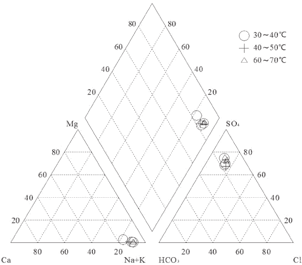
图 3 Piper 水化学类型三线图 [7] Fig.3 Three line diagram of hydrochemical types [7]
