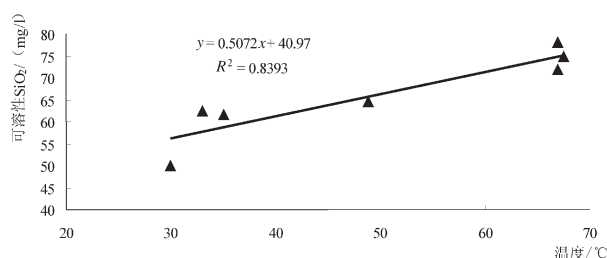
图2 地热流体中可溶性 \text{SiO}_2 含量与温度关系 Fig. 2 Relationship between content and temperature of \text{SiO}_2 of the geothermal fluid
