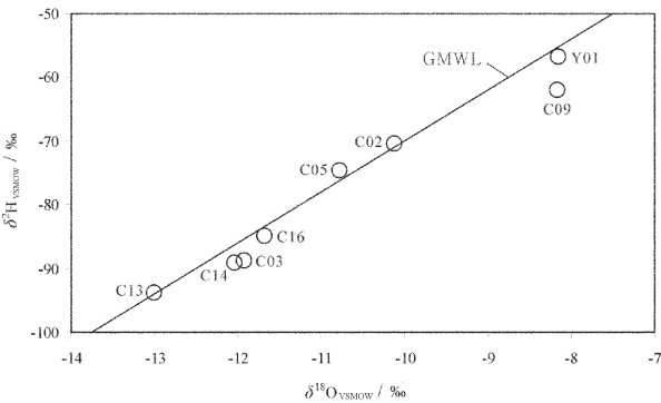
图 4 汤泉地区地热流体氢氧同位素特征 Fig.4 Hydrogen and oxygen stable isotope characteristics of the geothermal fluid in Tangquan area
