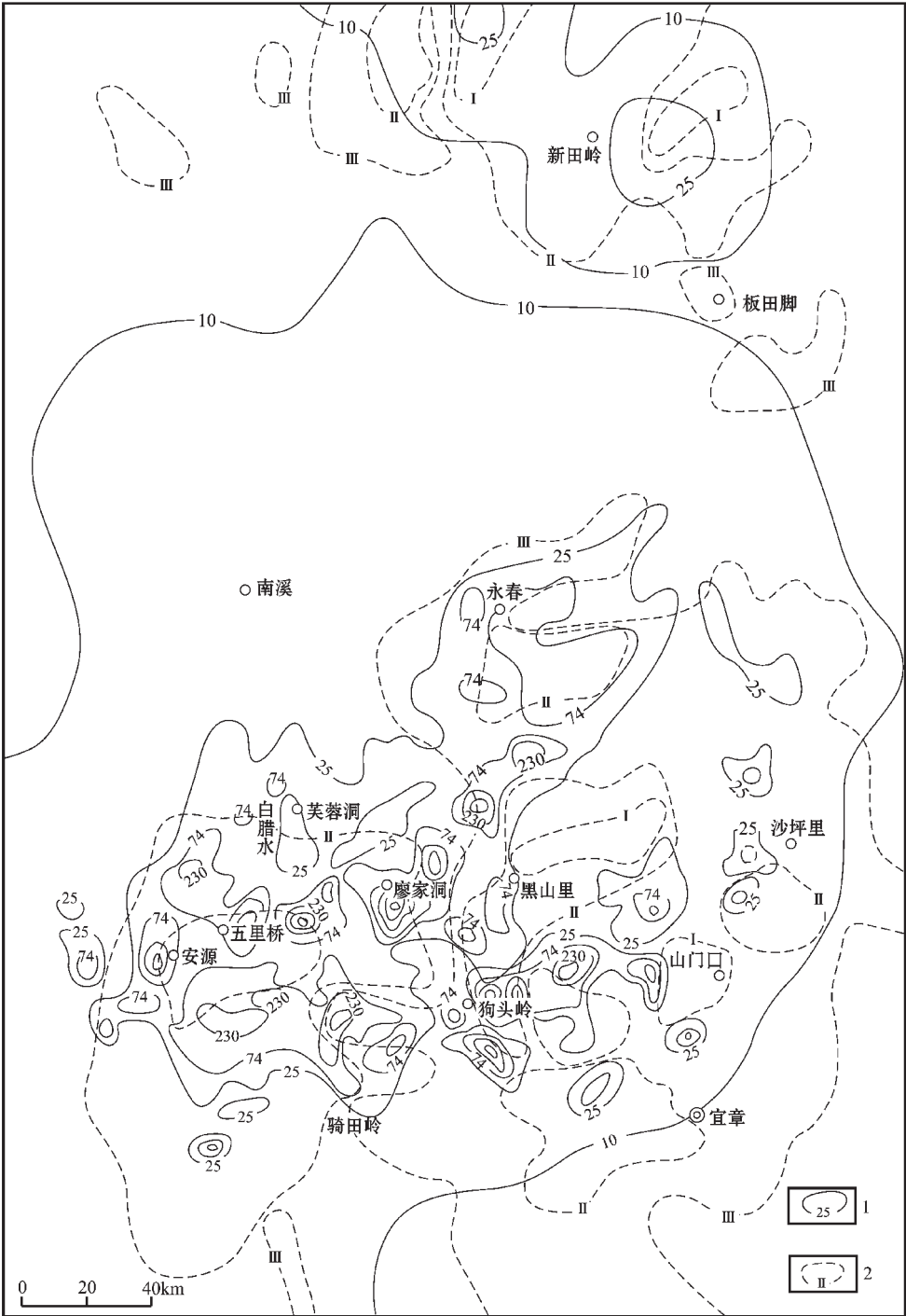
图4 骑田岭地区水系沉积物Sn异常和锡石重砂异常图 Fig. 4 Map showing the tin anomaly and cassiterite concentrate anomaly of stream sediments in the Qitianling area 1—水系沉积物Sn异常曲线 2—锡石重砂异常范围及级别
