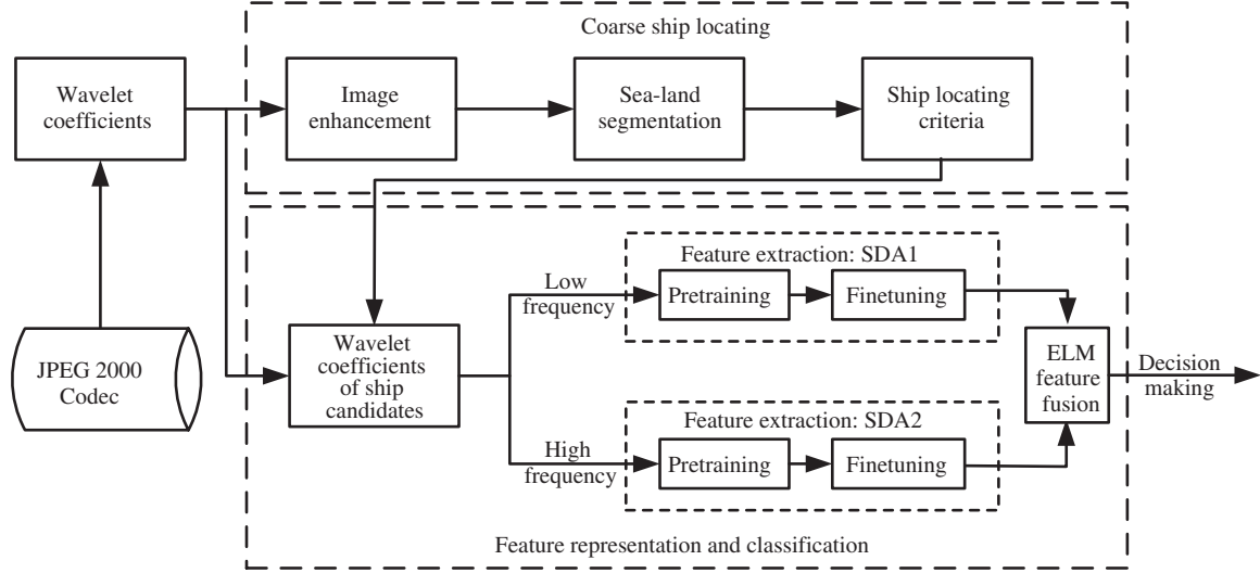
Figure 2 ELM-based ship detection framework.
