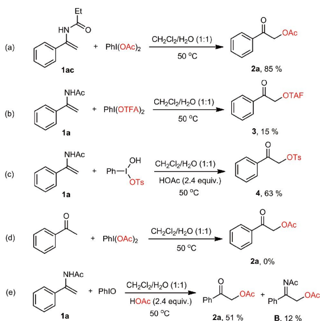
Scheme 4 Control experiments for studying the reaction mechanism (color online).
