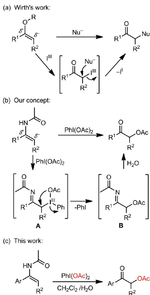
Scheme 2 Umpolung strategy for constructing of \alpha -acetoxy ketones.
