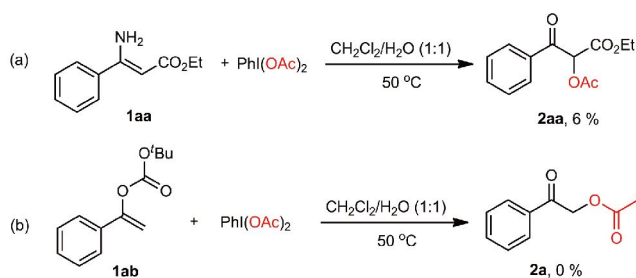
Scheme 3 Reaction of enamino esters, and enol carbonates with \text{PhI}(\text{OAc})_2 (color online).
