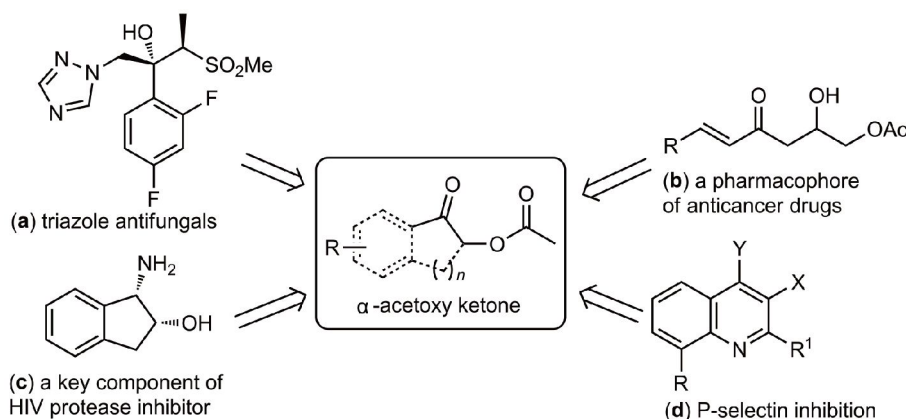
Scheme 1 \alpha -Acetoxy ketones as precursors for molecules of medicinal and biological importance.
