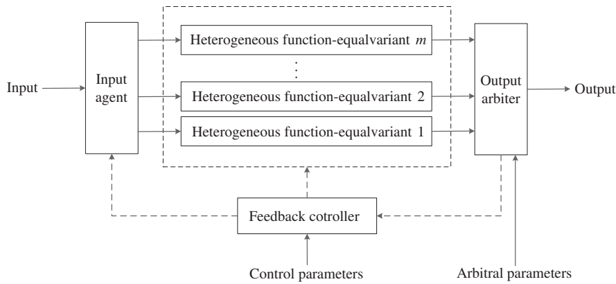
Figure 4 Abstract model of the mimic defense system.
