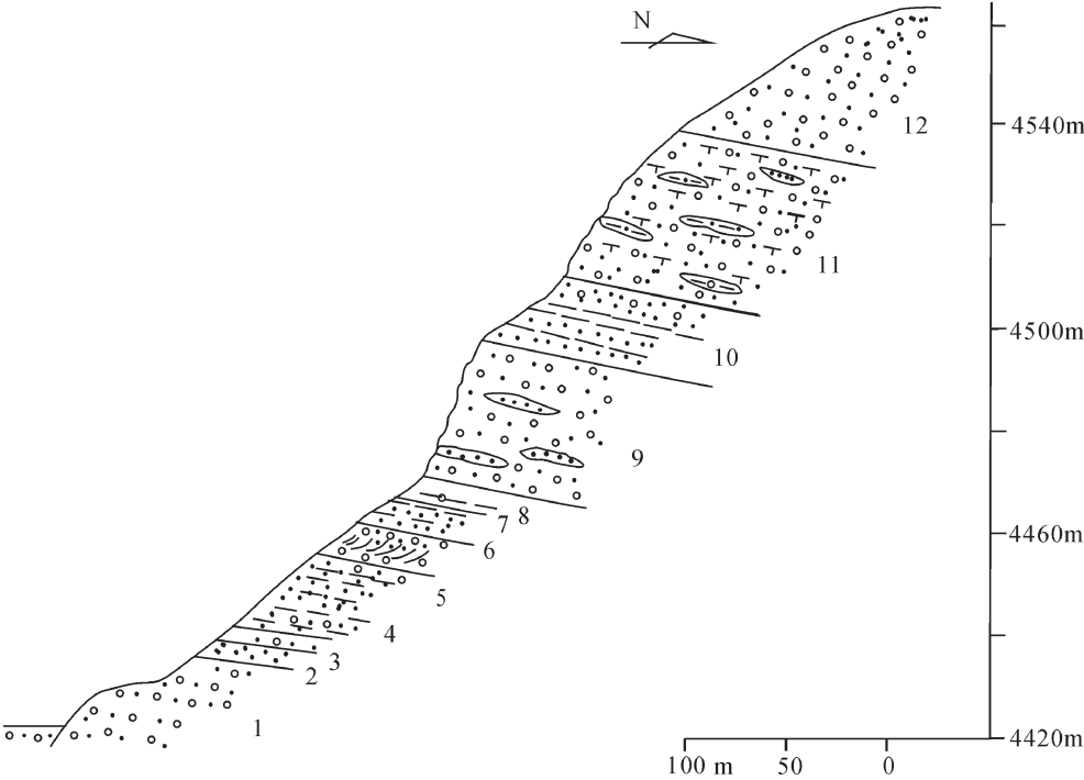
图 1 贡达甫村附近贡巴组剖面 Fig.1 Cross section of the Gongba Formation near Gongdapu Village, Tibet
