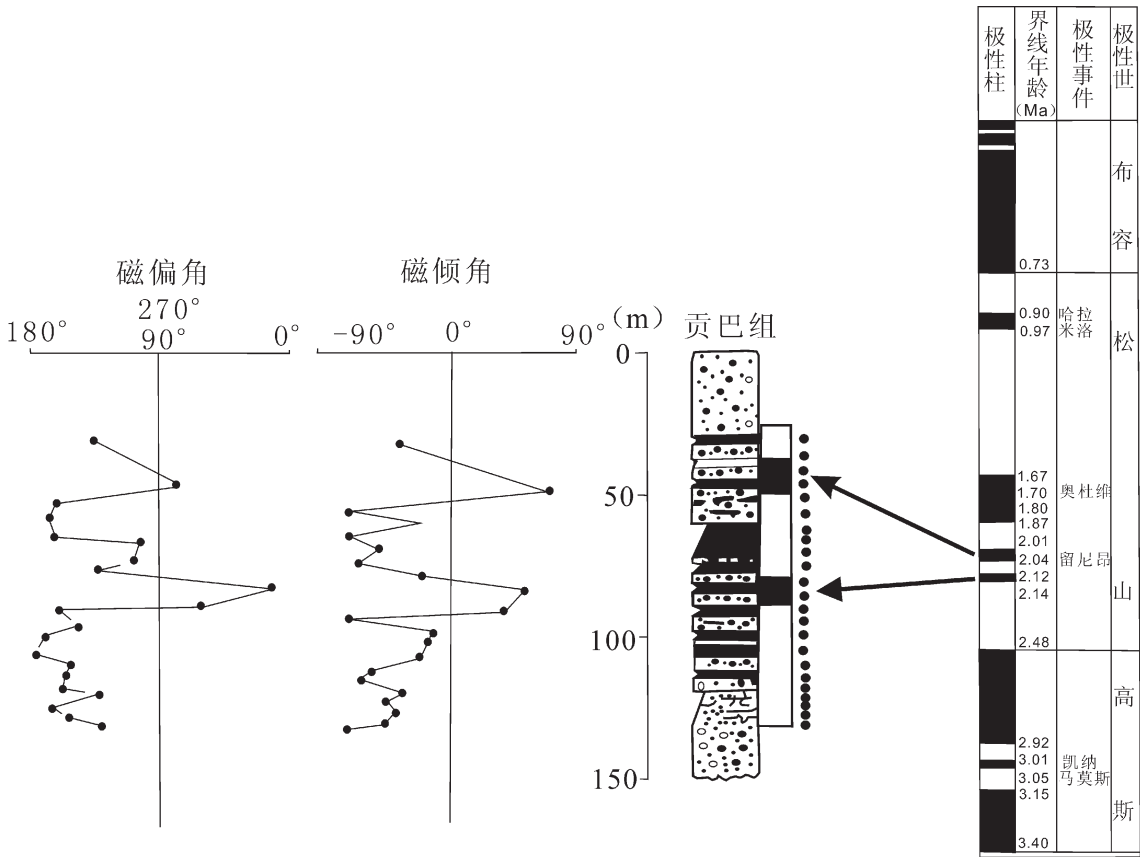
图 2 贡巴组地层剖面古地磁极性柱和极性年表对比图 Fig.2 Paleomagnetic polarity column of the Gongba Formation and correlation of the standard magnetic polarity chronological tables
