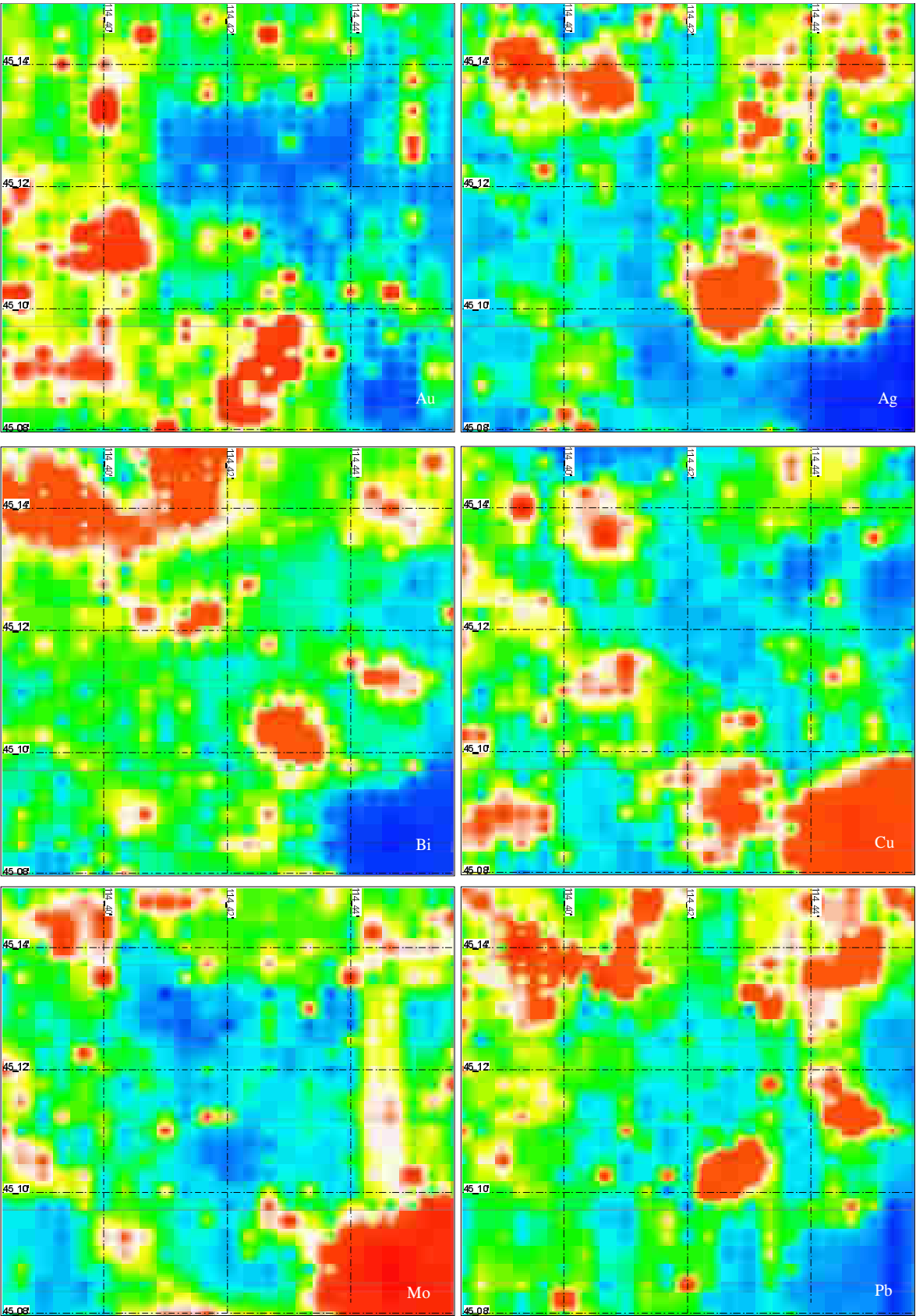
图 6 莫若格钦地区化探岩屑测量单元元素 Au, Ag, Bi, Cu, Mo, Pb 含量专题图 Fig.6 Thematic map of the elements Au, Ag, Bi, Cu, Mo and Pb in geochemical debris survey in the Moruoqeqin area
