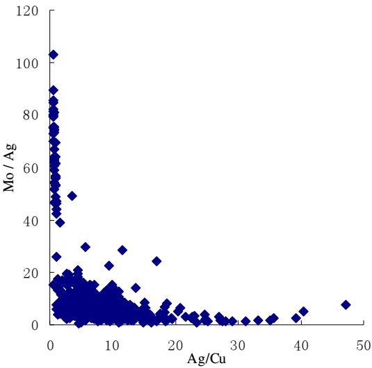
图 8 Mo/Ag 与 Ag/Cu 散点图(样品数 n=667); Fig.8 Scatter diagram of Mo/Ag vs. Ag/Cu (number of samples n=667)
