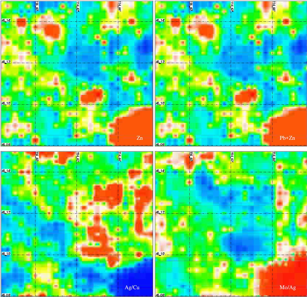
图 7 莫若格钦地区化探岩屑测量单元元素 Zn 及 Pb+Zn,Ag×1000/Cu 和 Mo/Ag×1000 专题图 Fig.7 Thematic map of the elements Zn and Pb+Zn, Ag×1000/Cu and Mo/Ag×1000 in geochemical debris survey in the Moruoqeqin area
