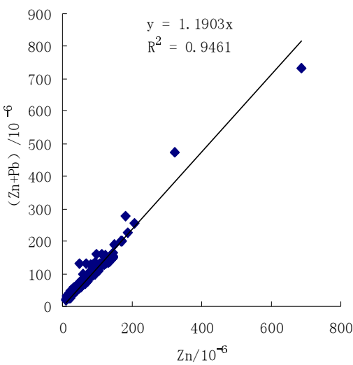
图 9 Zn+Pb 与 Zn 散点图(样品数 n=667) Fig.9 Scatter diagram of Zn+Pb vs. Zn (number of samples n=667)
