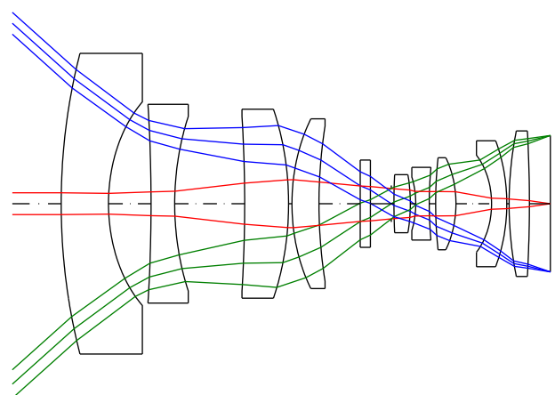
Figure 1. Structure diagram of the optical system.
