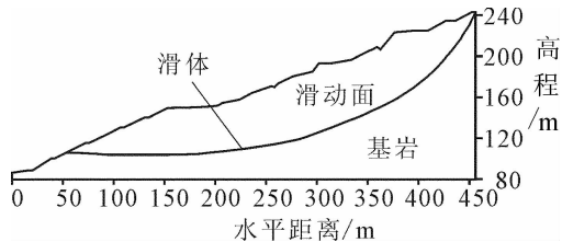
图 7 三峡库区某边坡剖面 Fig.7 Profile of a certain slope in the Three Gorges reservoir area
