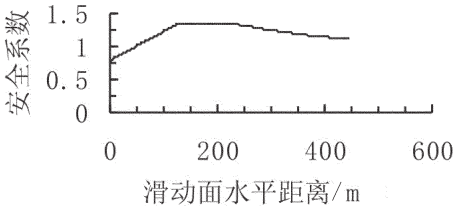
图 9 三峡库区某边坡沿滑动面的安全系数 Fig.9 Safety factor along the failure surface of a slope in the Three Gorges reservoir area
