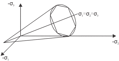
图 1 摩尔-库仑屈服面(多边形)和 D-P 屈服面(外接圆) Fig.1 Yield surface for D-P and Mohr-Coulomb
