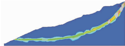
图 10 三峡库区某边坡沿滑动面的塑性主剪应变 Fig.10 Principal plastic shear strain along the failure surface of a slope in the Three Gorges reservoir area
