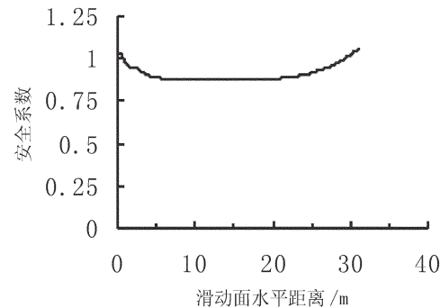
图 6 沿滑动面的安全系数 Fig.6 Safety factor along the failure surface of the slope
