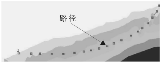
图 8 初始 c 、 \varphi 值时,三峡库区边坡应力等值线和路径 Fig.8 Stress contours and path of the slope in the Three Gorges reservoir area at the initial c and \varphi
