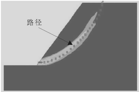
图 2 滑动面和路径 Fig.2 Failure surface and path
