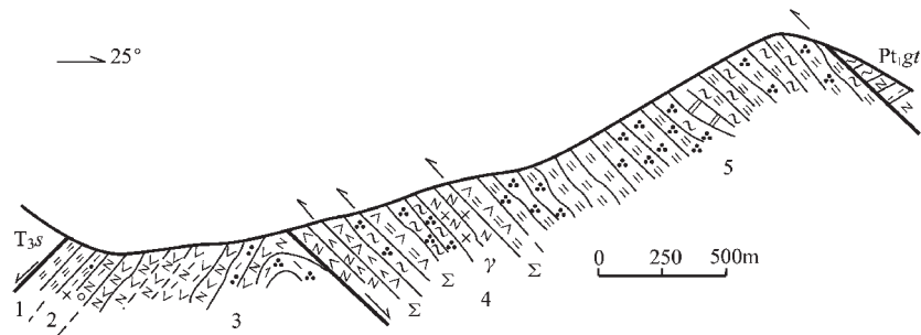
图2 李子坪蛇绿混杂岩剖面 Fig. 2 Geological section of the Liziping ophiolitic melange in Yangbi County, Yunnan Province
