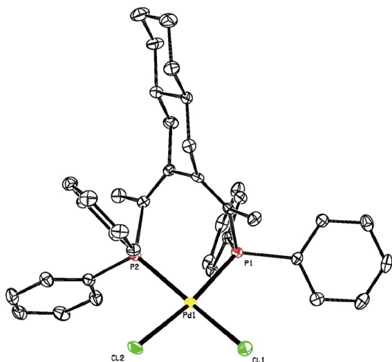
Figure 2 X-ray structure of \text{Pd}(\text{L3})\text{Cl}_2 (color online).
