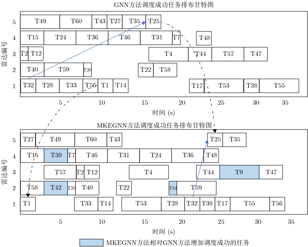
图 10 两种GNN模型对相同实例的成功调度结果甘特图对比 Fig. 10 Comparison of successfully scheduling results gantt charts of two models on the same instance
