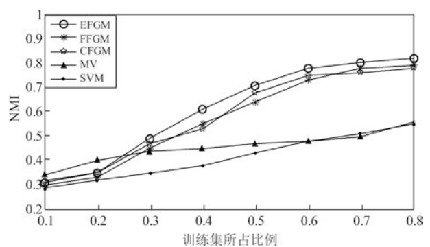
图 4 训练集所占比例对 NMI 指标的影响 Fig. 4 The impact of the training set percentage on NMI score
