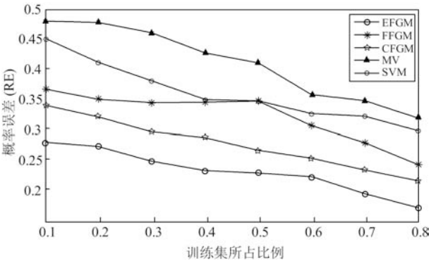
图 5 训练集所占比例对概率误差的影响 Fig. 5 The impact of the training set percentage on RE score
