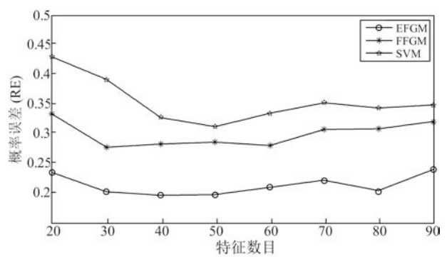
图 3 特征数目对概率误差的影响 Fig. 3 The impact of the number of features on RE score
