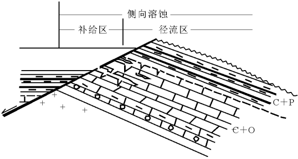
图 2 断裂活动对储集空间的改造作用示意 Fig. 2 The scheme of reservoir space reconstruction caused by fracturing
