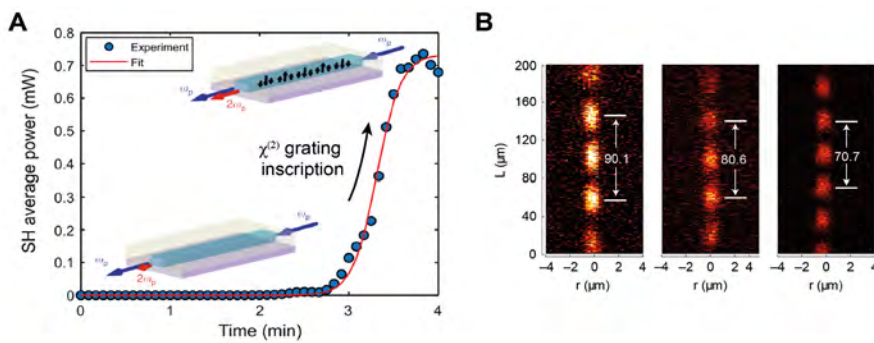
Figure 3. (a) Experimental SH power generated during all-optical poling. The inscription of the grating in a SiN waveguide results in a fast build-up of SH light [9]. (b) Two-photon microscopy images of inscribed gratings in a SiN microring. Depending on the probed resonance, the grating period automatically adapts to guarantee phase matching [10]. (c) Picture of a SiN microring under operation after all-optical poling showing SH light generation.
