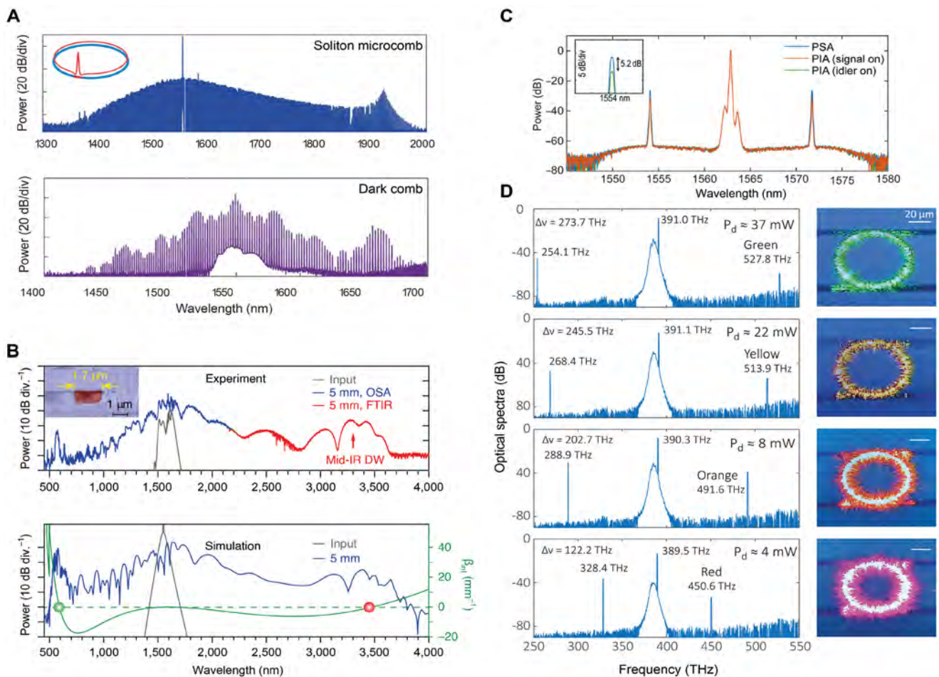
Figure 2. (a) Examples of soliton microcombs generated in SiN microrings. Top spectrum represents a bright soliton, bottom one a platicon state (dark soliton) [2]. (b) SCG in a 5 mm dispersion engineered SiN waveguide. Widely spaced dispersive waves (DW) are observed near the zero-integrated dispersion points around 600 and 3500 nm, in agreement with simulation [5]. (c) Experimental demonstration of CW parametric amplification from a SiN waveguide [6]. (d) OPO in a SiN microring enabling the coherent generation of visible/near visible light on chip, tunable by adjusting the pump wavelength (around 390 THz) [8].
