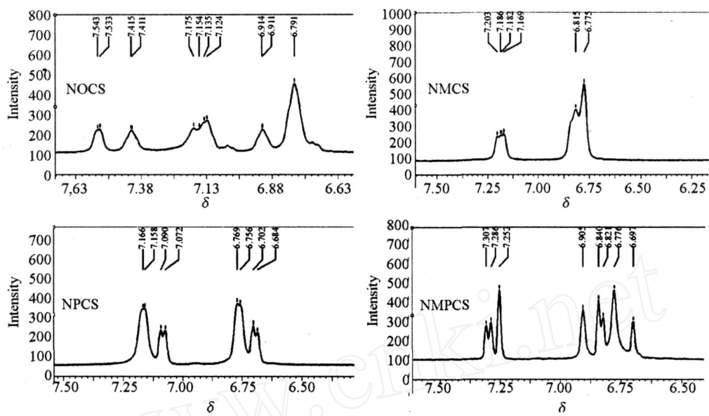
图 3 N-苄基壳聚糖衍生物的核磁共振氢谱 Fig.3 ^1\text{H} -NMR spectra of N-benzyl chitosan derivatives
