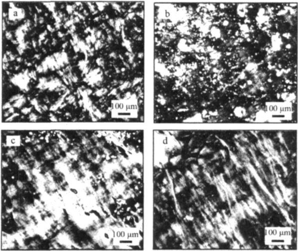
图 4 N-苄基壳聚糖衍生物甲酸溶液的偏光显微镜照片 a. \omega(\text{NOCS}) = 39\% ;b. \omega(\text{NMCS}) = 41\% ; c. \omega(\text{NPCS}) = 39\% ;d. \omega(\text{NMPCS}) = 39\% Fig. 4 POM photographs of N-benzyl chitosan derivatives/ formic acid solutions
