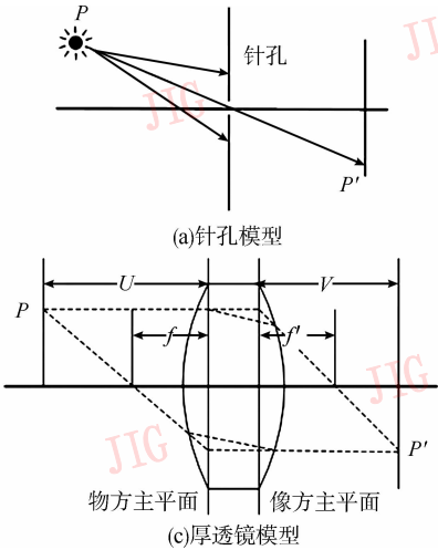
Fig. 2 Optical imaging principle of camera lens models
