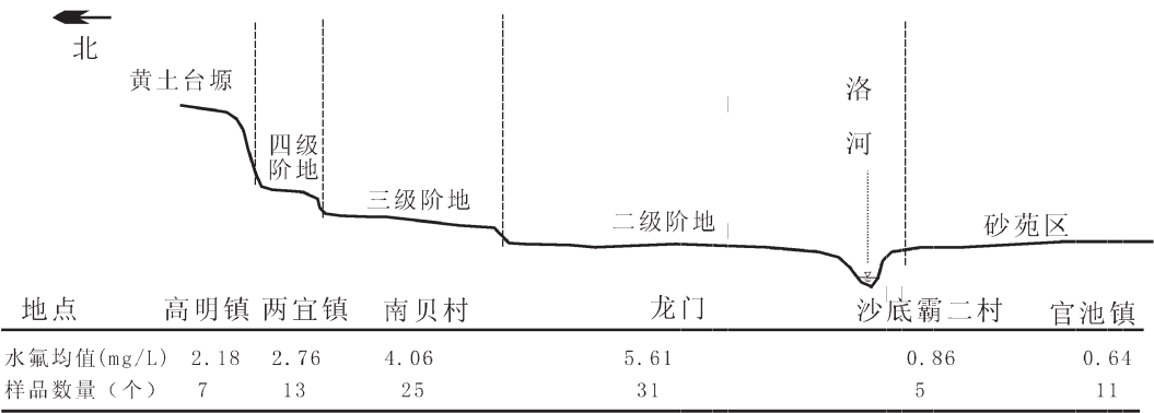
图 4 大荔县地貌与水氟的关系分析示意图 Fig.4 The relationship between geomorphology and water fluoride in Dali County
