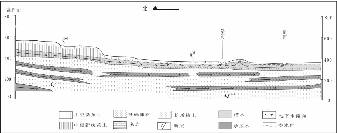
图 1 大荔县水文地质剖面图 Fig.1 Hydrogeological profile of Dali County
