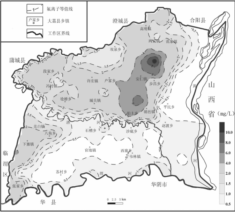
图 3 大荔县潜水中氟离子等值线图 Fig.3 Contour map of fluoride in phreatic water of Dali County
