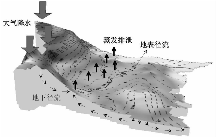
图 2 大荔县地下水水循环示意图 Fig.2 Schematic map showing cycling of groundwater in Dali County
