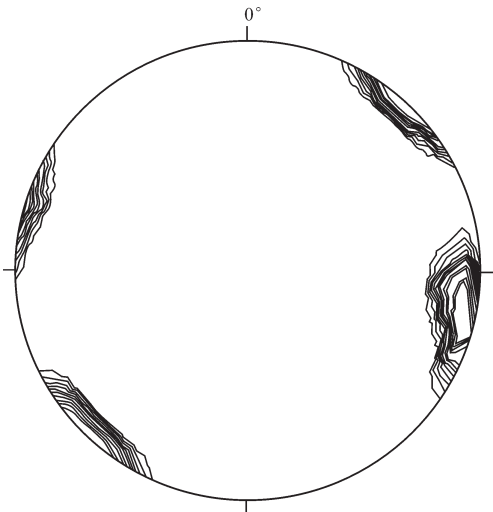
图 7 主应力的等密线图 Fig.7 Pole isodensity diagram of the principal stress
