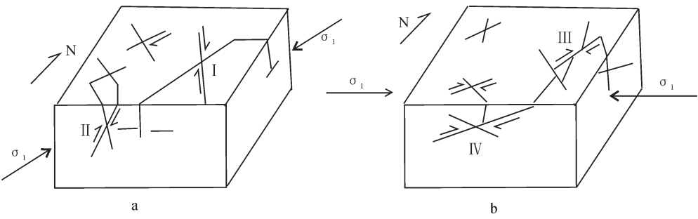
图 8 金川坝址区节理构造模拟演化图 Fig.8 Simulation of the evolution of joints in the Jinchuan dam area
