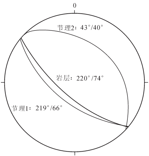
图 9 层面与节理关系赤平投影图 Fig.9 Stereographic projection of the relationship between the beds and joints
