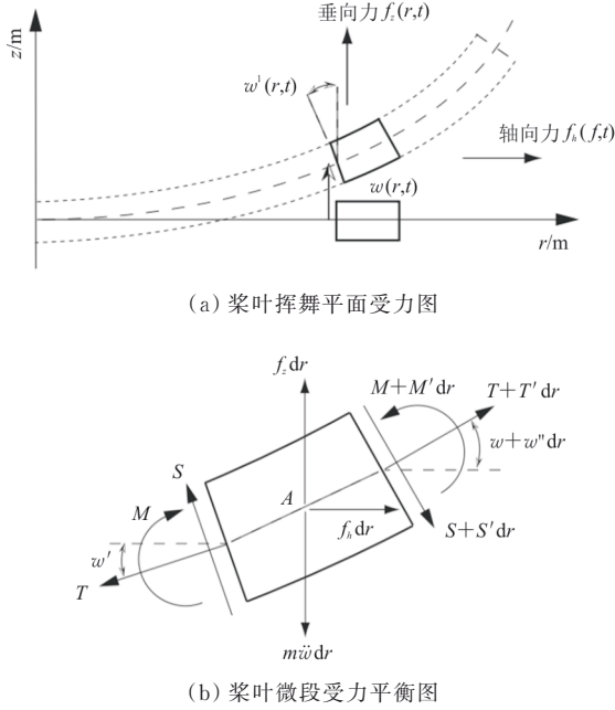
图2 挥舞面内桨叶微段受力图 Fig. 2 Microsegment force diagram of blade in flapping plane
