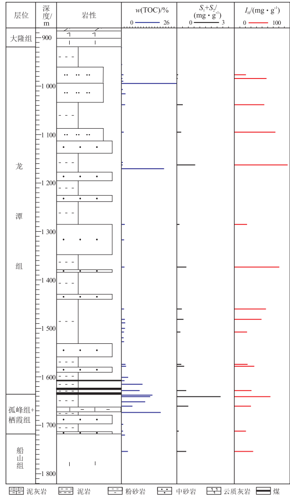
图8 南黄海地区 CSDP-2 井地化综合柱状图 Fig.8 Geochemical column of well CSDP-2, South Yellow Sea
