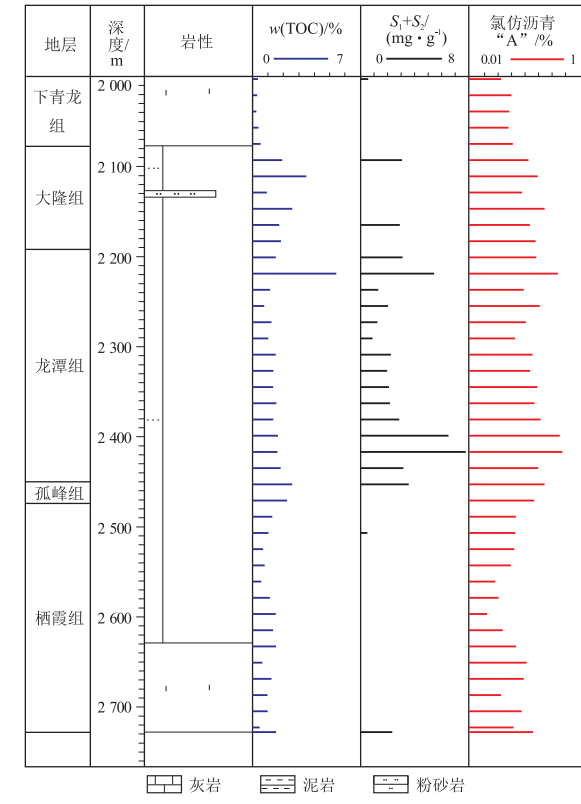
图9 南黄海地区 CZ35 井地化综合柱状图 Fig.9 Geochemical column of well CZ35, South Yellow Sea
