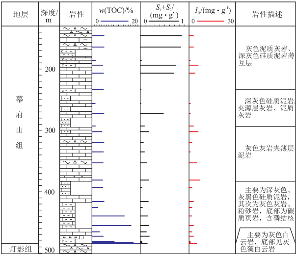
图 4 江苏盱眙 GuanD1 井下寒武统幕府山组烃源岩地化综合柱状图 Fig.4 Geochemical column of source rocks in Lower Cambrian Mufushan Formation in well GuanD1, Xuyi, Jiangsu province
