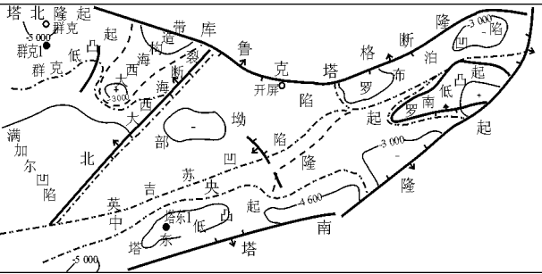
图6 塔里木盆地东北部古生界构造区划示意 [52] Fig. 6 A simplified structural map of the northeastern Tarim Basin, showing Paleozoic structures [52]
