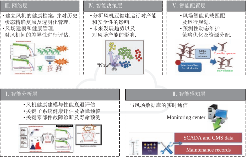
图 9 基于 CPS 的 5C 架构体系的智能化风力发电风场 Fig.9 The flow of data and information in a 5C architecture based wind farm
