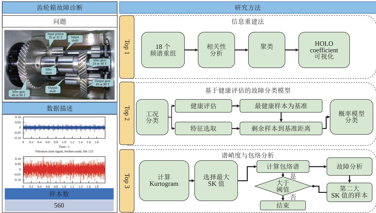
Fig.4 2009 PHM data competition fault diagnosis of gearbox
