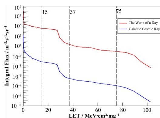
图1 ASO-S轨道宇宙线重离子LET积分谱 Fig.1 LET integral spectrum of cosmic ray heavy ions in ASO-S orbit
