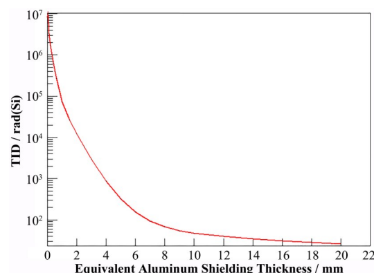
图2 ASO-S轨道上的总剂量-屏蔽厚度关系曲线 Fig.2 Relationship curve between total dose and shield thickness in ASO-S orbit
