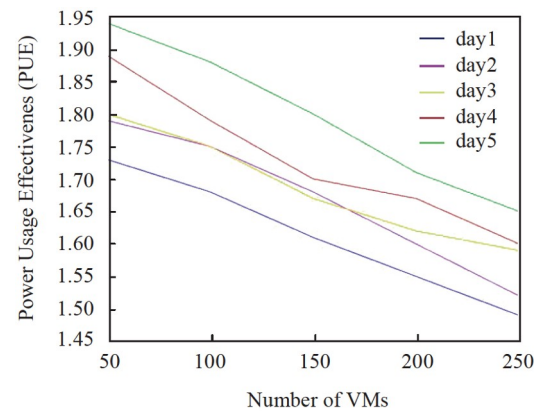
Figure 6 Power usage effectiveness during five days of operation of the reinforcement cloud system in CloudSim.
